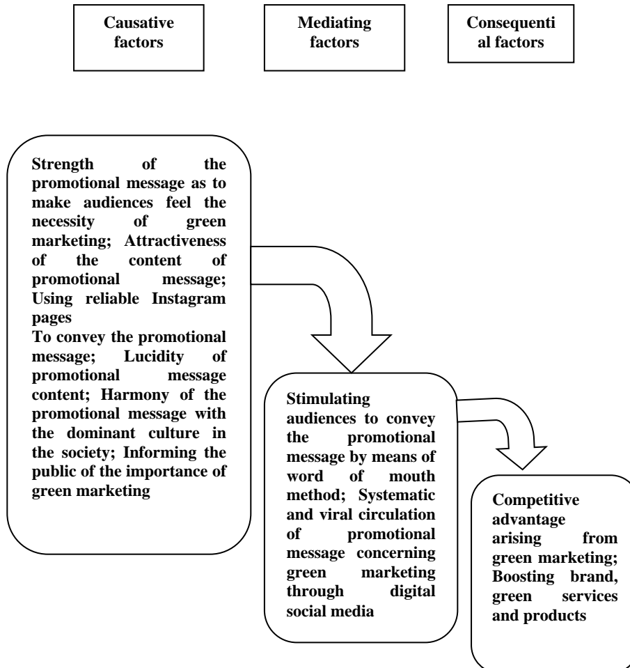
Fig.3.The proposed model
