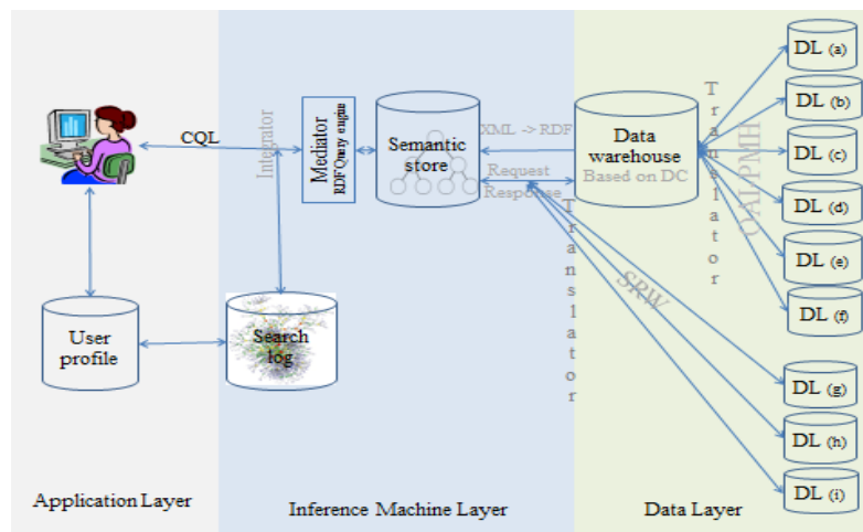
Figure 3. Proposed architecture facilitating semantic integration in heterogeneous DLs
